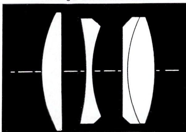
Agfa Color-Solinar 1:2,8/50 mm
