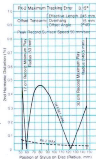
Horizontal Tracking Error vs. Harmonic Distortion
