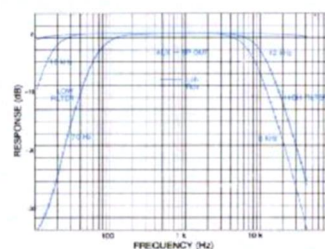
Filter Characteristics
