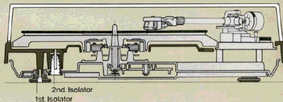
Cross section of SL-1301
