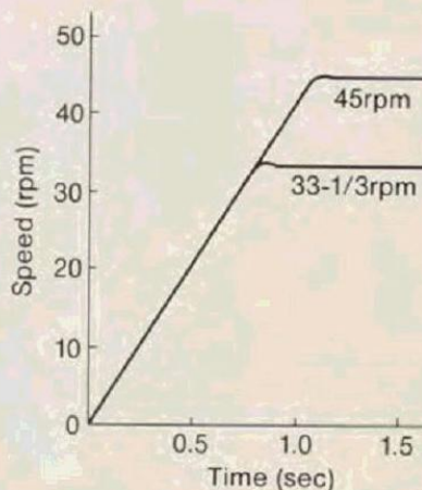
Start-up time
