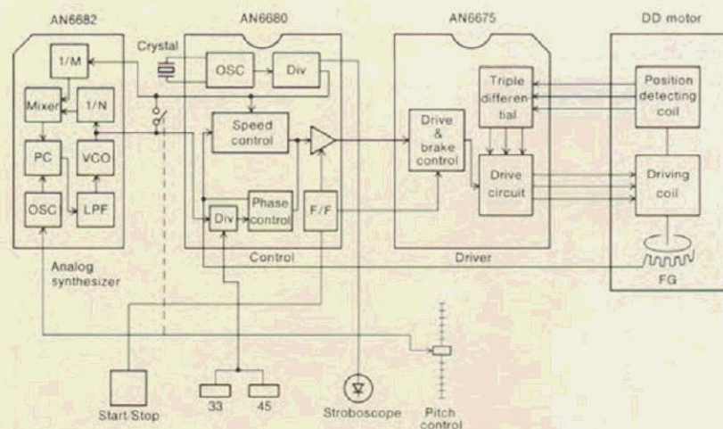
Block diagram
