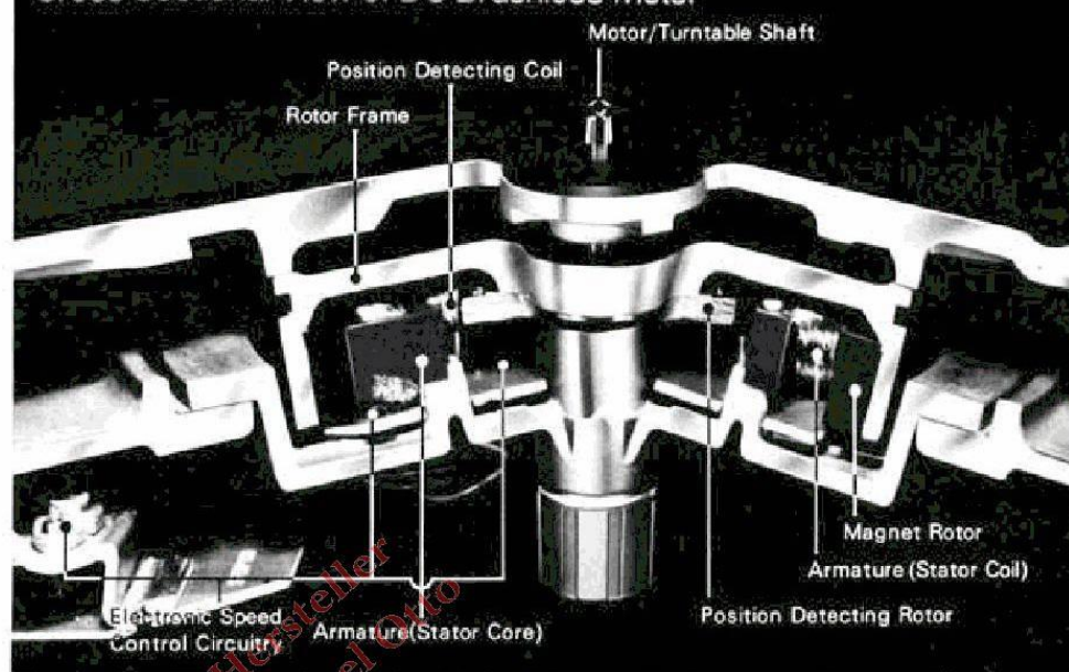
Cross Sectional View of DC Brushless Motor
