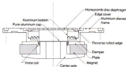
8 cm Honeycomb Disc Midrange
