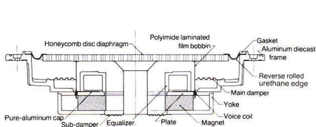
32 cm Honeycomb Disc Woofer
