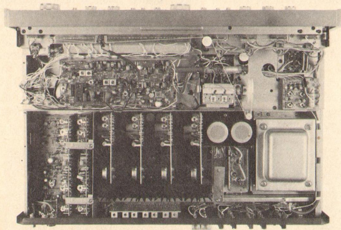
Fig. 2—Internal view.
