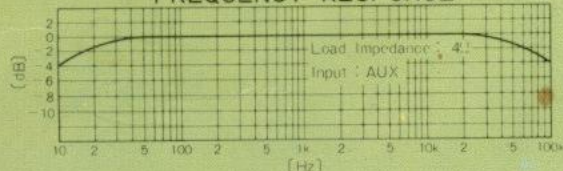
FREQUENCY RESPONSE
