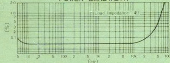
POWER BANDWIDTH
