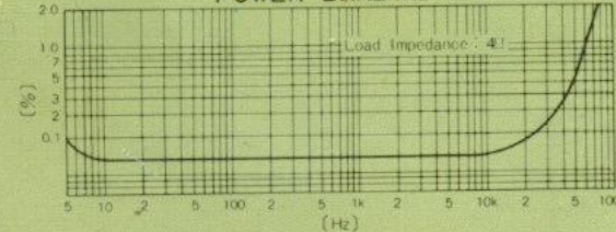
POWER BANDWIDTH
