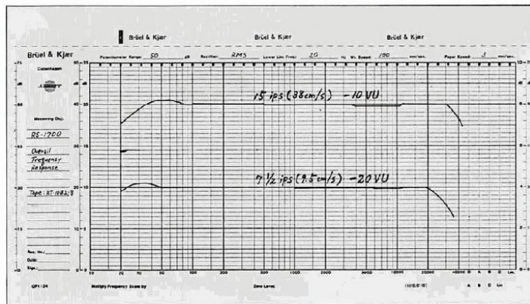
Overall Frequency Response
