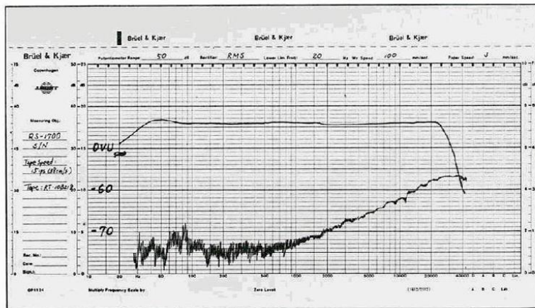
Signal-to-Noise Characteristics
