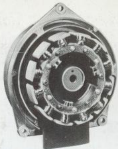
Wickelteller motor
