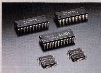
MASH-1-Bit-D/A-Wandler-LSIs
