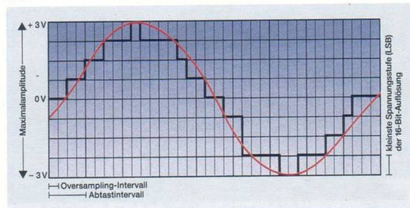
16-Bit/4-fach-Oversampling
