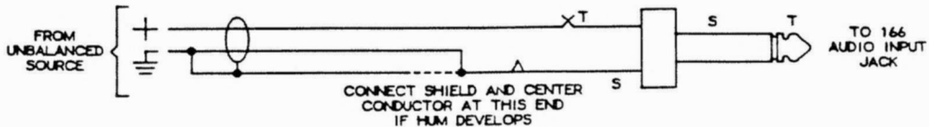
Figure 3b: Same, mono plug
