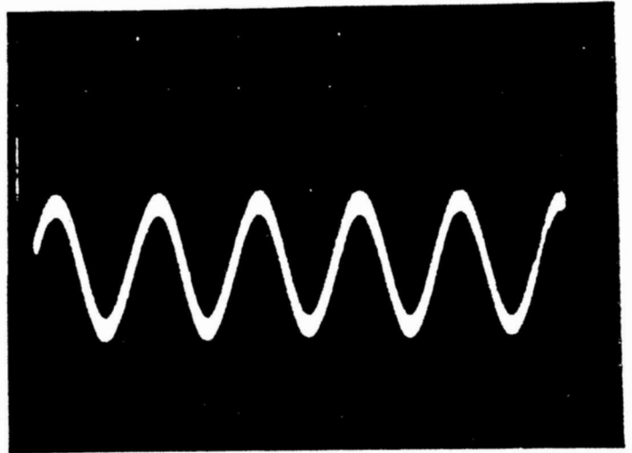
Figure B. TP1 (TP5) After Adjusting R34 (R154) for peaks at 0 vdc. (1mV/div, DC coupled)
