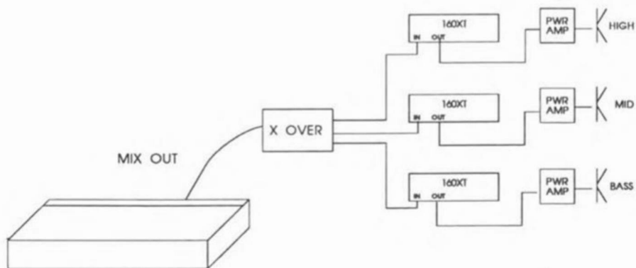
Figure 7: Connecting 160XTs for Sound Reinforcement
