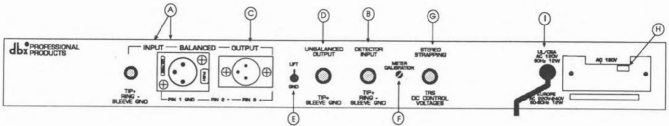
Figure 3: Rear Panel
