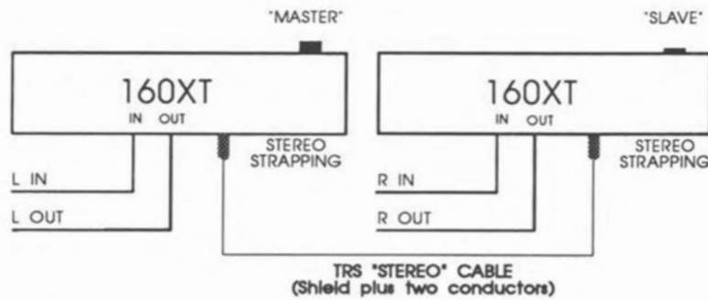
Figure 8: Multi Channel Connections
