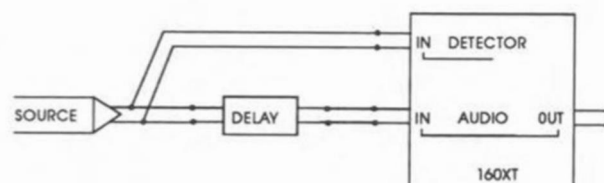
Figure 16: Anticipated Compression
