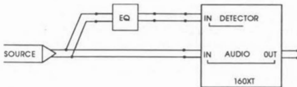
Figure 15: Frequency-Weighted Compression
