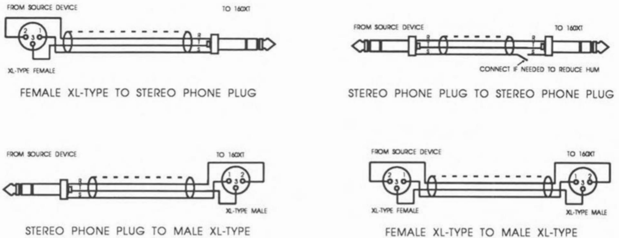
Figure 17: Input Connections (Balanced Lines)
