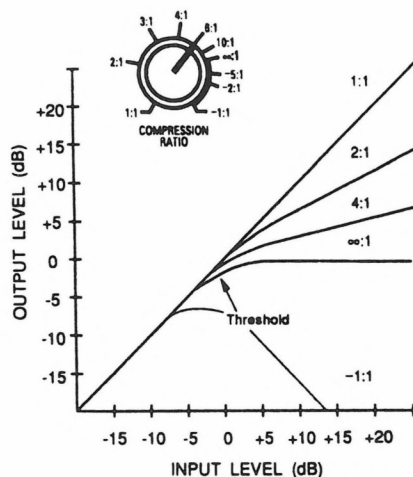
Figure 3: Ratio Control and Infinity+ (Negative) Ratios
