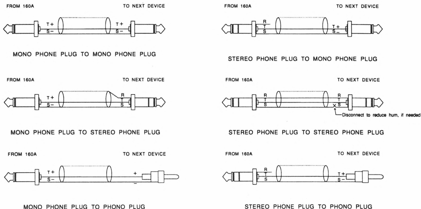
Figure 11: Output Connections (Unbalanced Operation)
