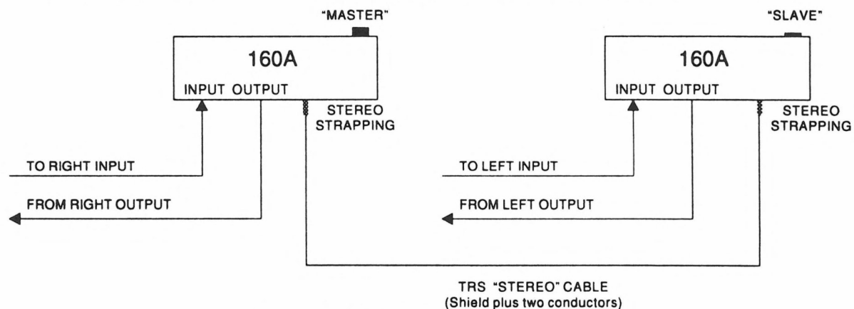
Figure 6: Multi-Channel Connections
