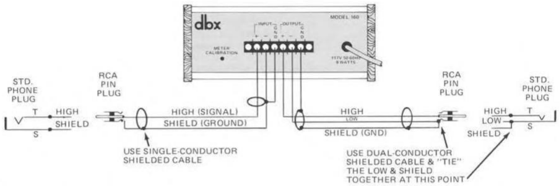
Fig. 2B - Connecting the 160 in an Unbalanced Circuit
