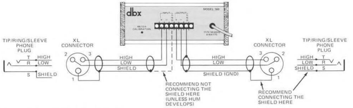
Fig. 2A - Connecting the 160 in a Balanced Circuit
