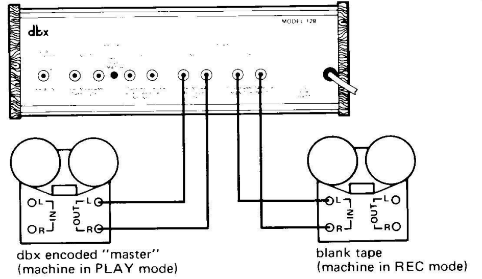
Fig. 11 – Making a Non-Encoded Copy from dbx-Encoded Master without a Preamp.
