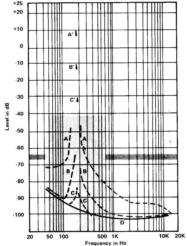
Fig. 17 – Tape Noise Characteristics (description next page)
