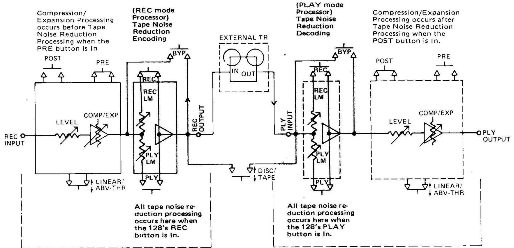
Fig. 14 – Signal Flow Diagram
