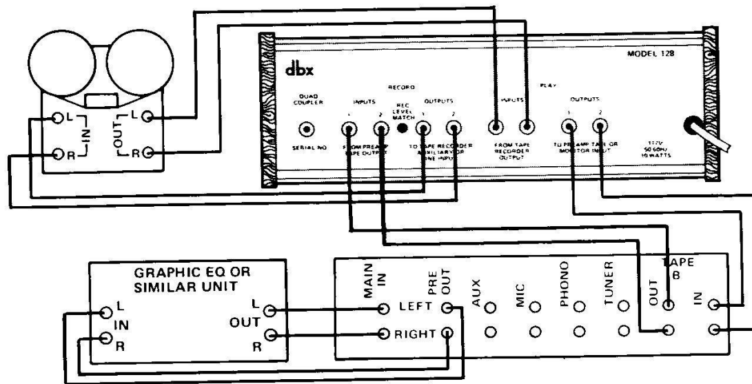
Fig. 6 – Where to Connect a Graphic Equalizer, Electronic Crossover, Reverb, Matrix 4-Channel Decoder, Etc. (Special signal processing follows the dbx encode/decode process.)
