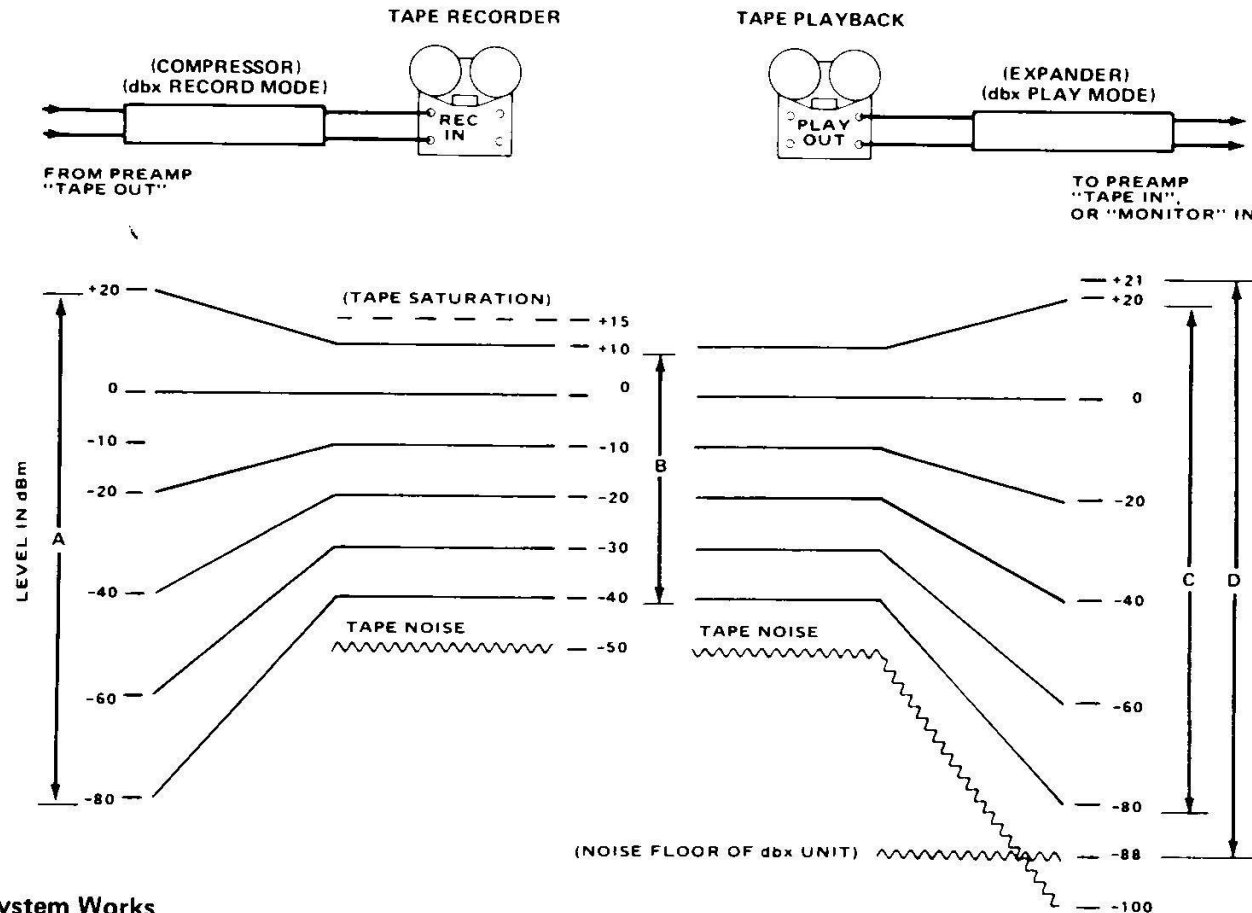
Fig. 15 – How the dbx System Works
