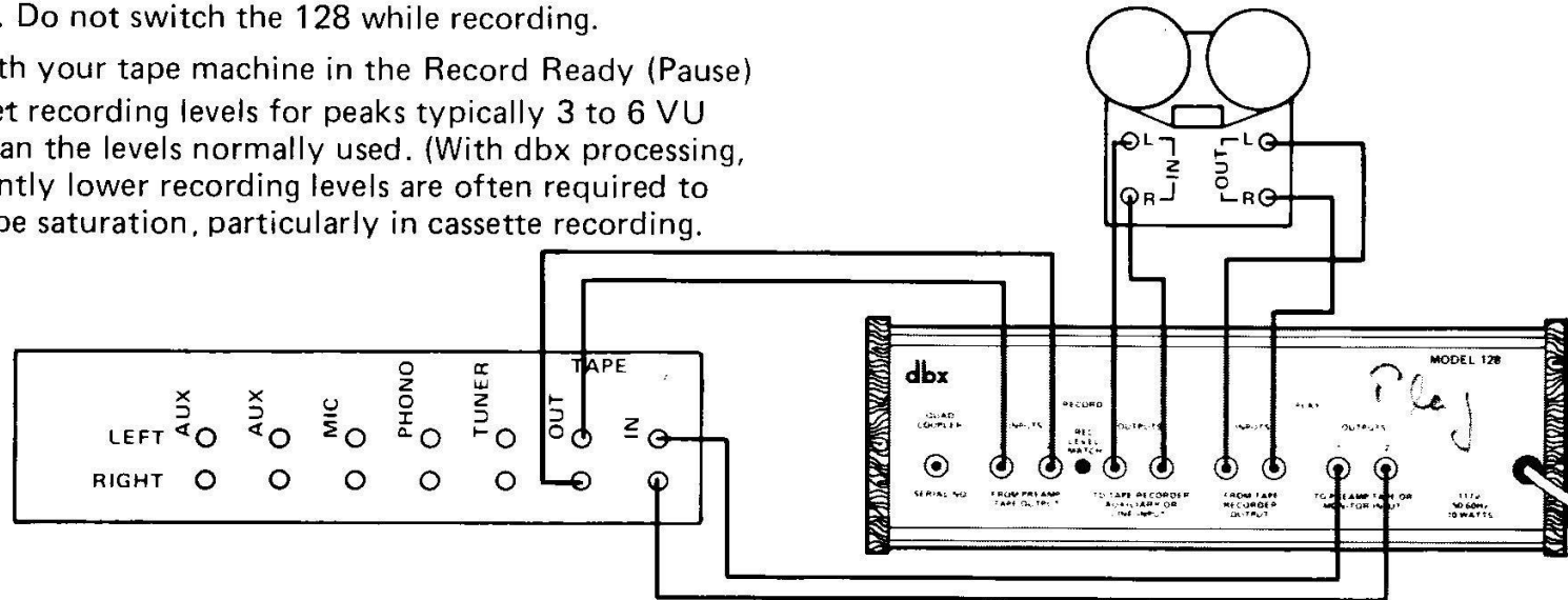
Fig. 3 – Basic Hook-Up Diagram
