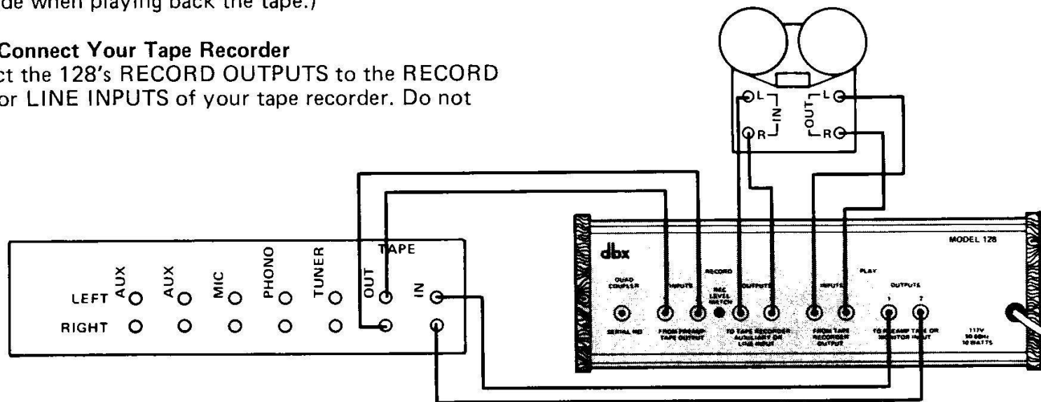
Fig. 4 – Connecting the 128 in a Tape Monitor Loop
