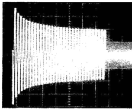
Fig. 2: Model 117 output with compression factor 1.4.
