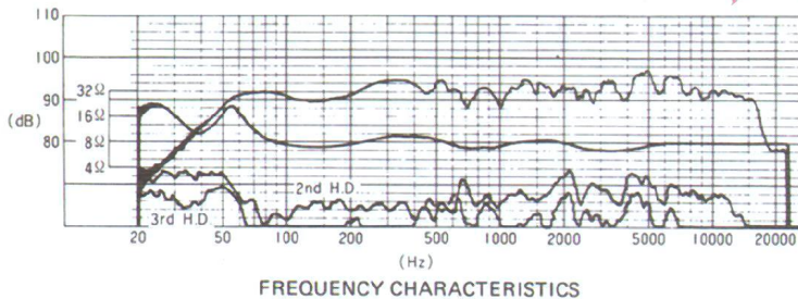
FREQUENCY CHARACTERISTICS
