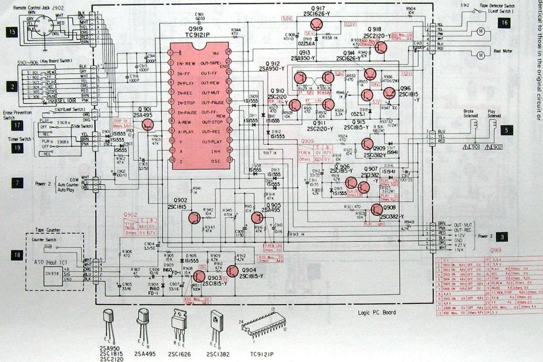
■ SCHEMATIC DIAGRAM (LOGIC BLOCK)
