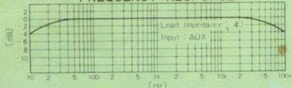
FREQUENCY RESPONSE
