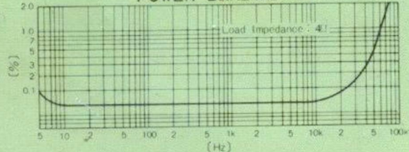
POWER BANDWIDTH
