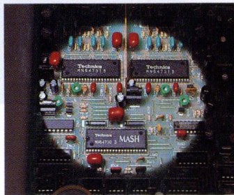
MASH-1 Bit-D/A-Wandler-LSIs
