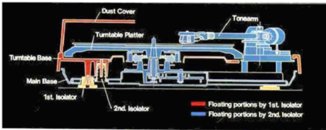
Double Isolated Suspension System
