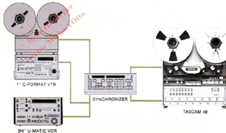
Audio production multiple machine system.
