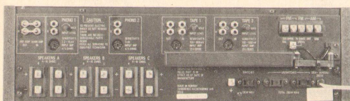
Fig. 1—View of back panel.
