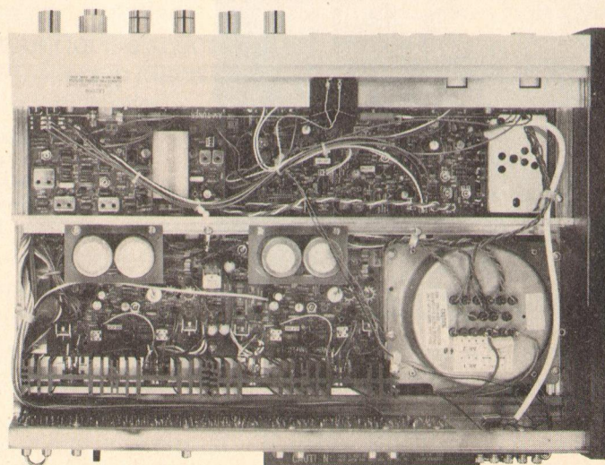
Fig. 2—Internal view.
