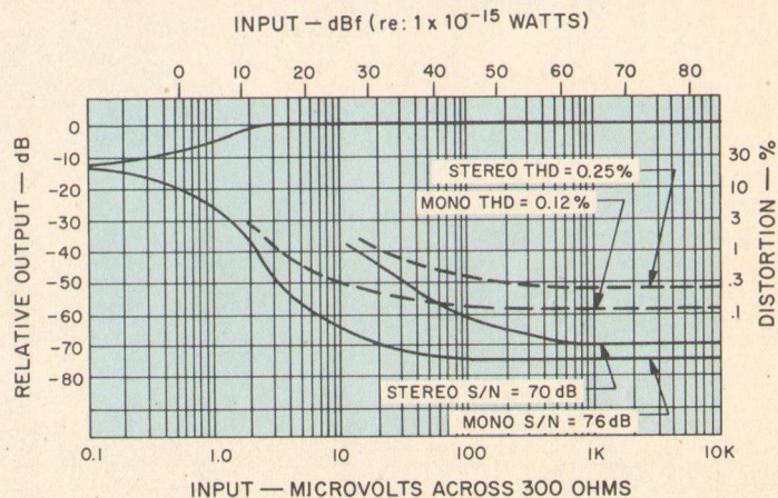
Fig. 4—FM quieting and distortion characteristics.
