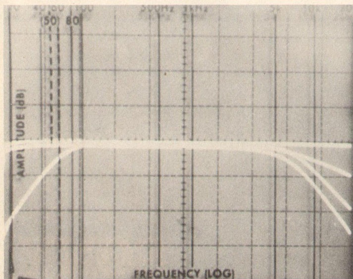
Fig. 11—Low- and high-cut filter combinations.
