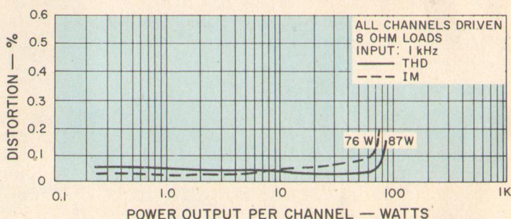
Fig. 8—Total harmonic and intermodulation distortion characteristics.
