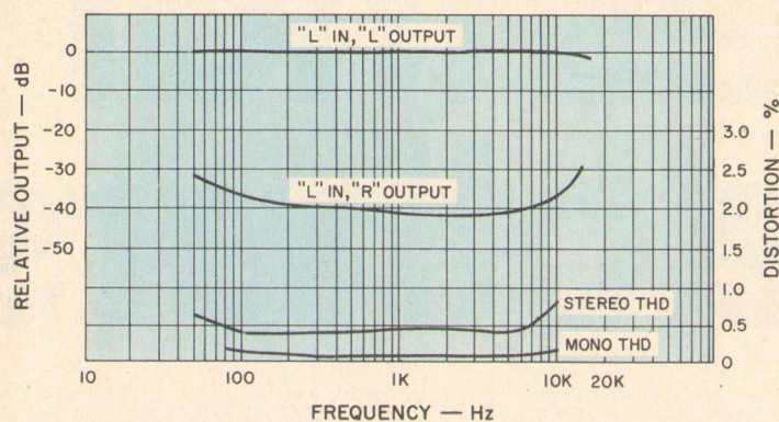
Fig. 5—Separation and distortion versus frequency.
