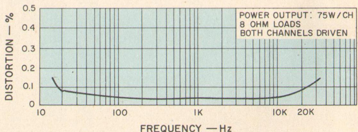
Fig. 9—Total harmonic distortion versus frequency.
