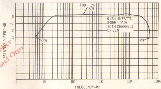
Fig. 7—Power bandwidth
