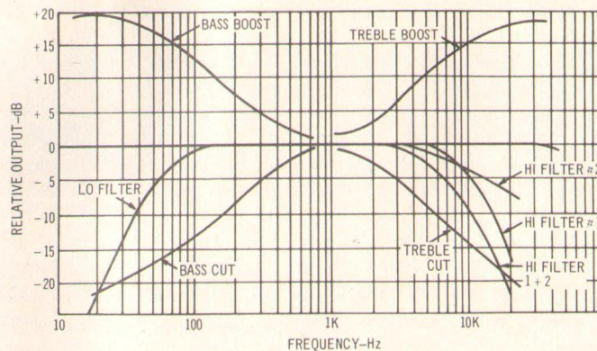
Fig. 8—Tone control and filter curves
