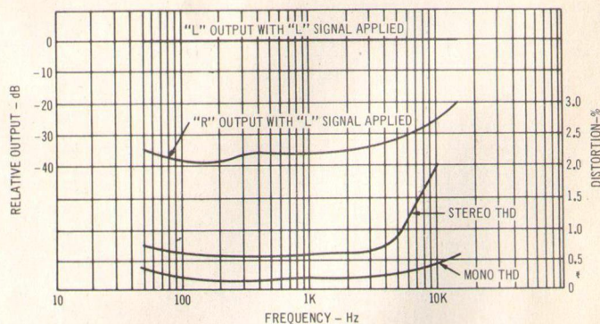
Fig 4—Separation, stereo and mono distortion.
