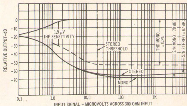
Fig 3—FM performance
