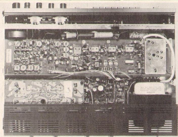
Fig 2—Inside view
