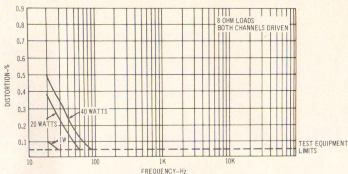
Fig. 6—THD v frequency
