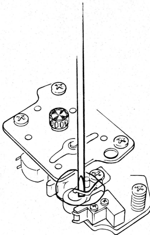
Fig. 3.3 Changing the pinch rollers
