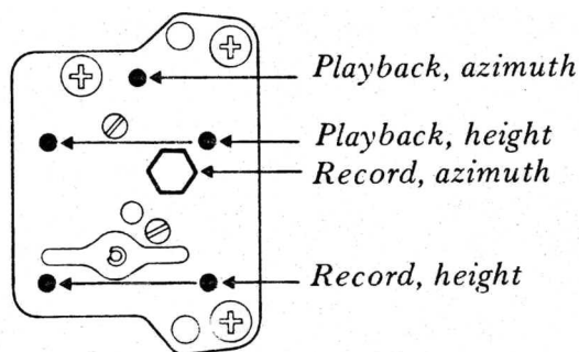
Fig. 5.6 Adjustments for the heads
