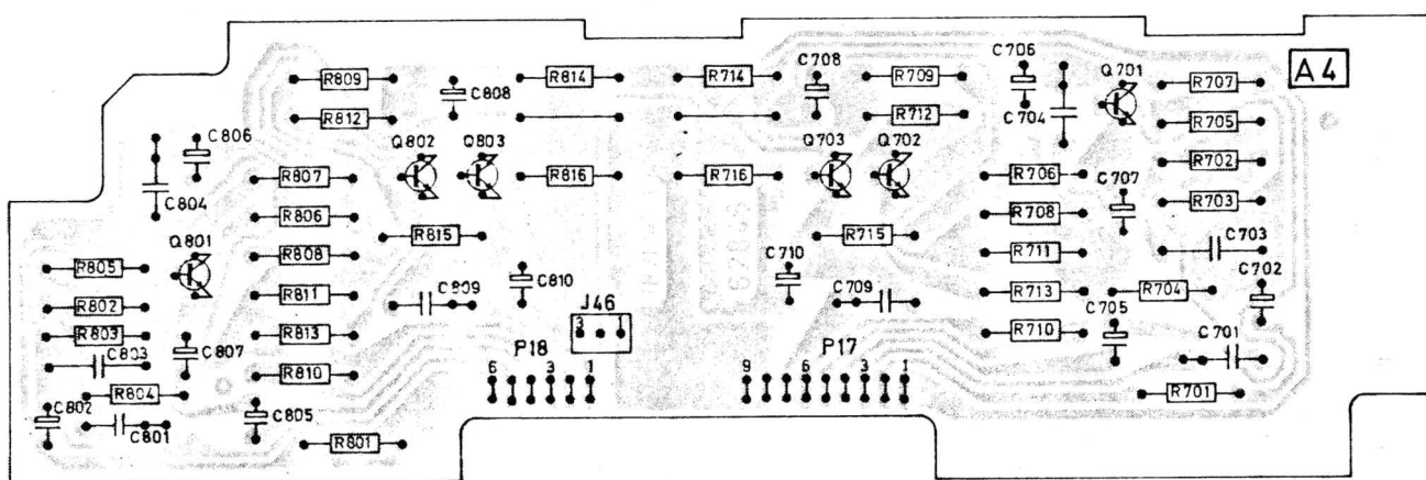
A4 EQUAL REC. AMP.
