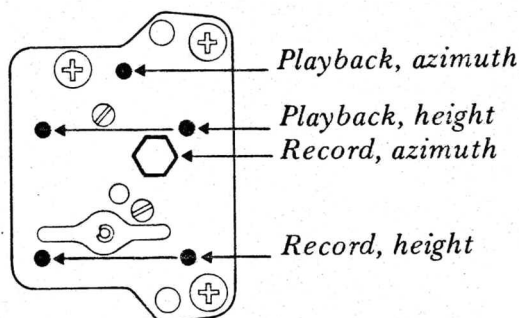
Fig. 6.3 Adjustments for the heads
