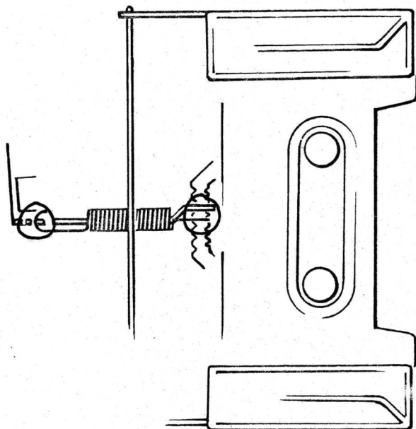
Fig. 3.7 Spring for headbridge
