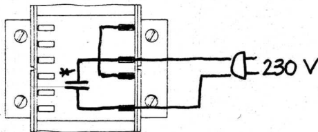
Powertransformer, part No. 352622, UI 48/26 TD2600
