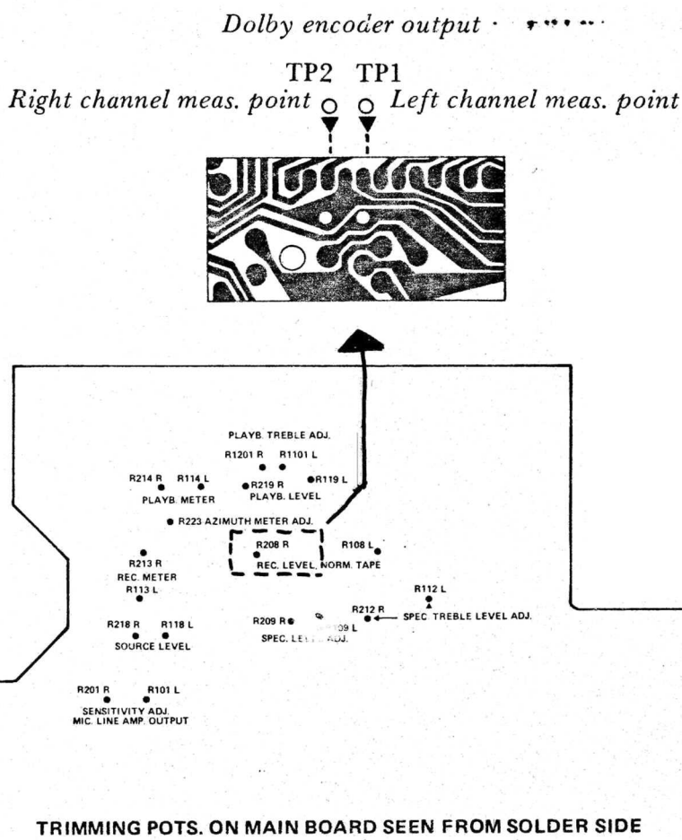
Fig. 6.1 Trimming pots. and Dolby encoders measurement points
