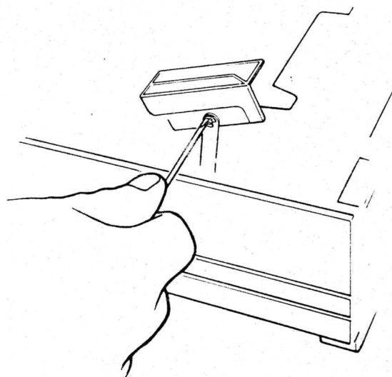
Fig. 3.2 Removing the circlip on the locking arm
