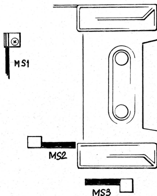
Fig. 3.14 Spring contacts
