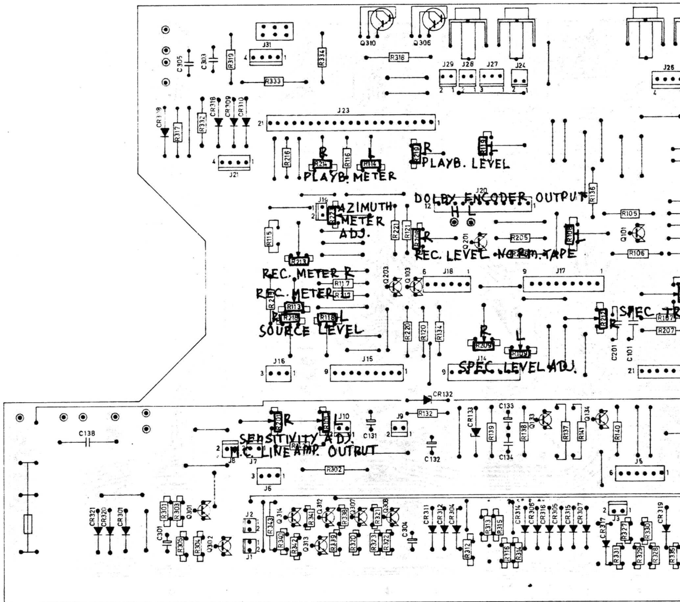
A1 MAIN BOARD
