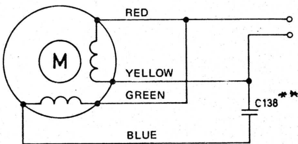
Capstanmotor, part No. 283767, HU 443AG
