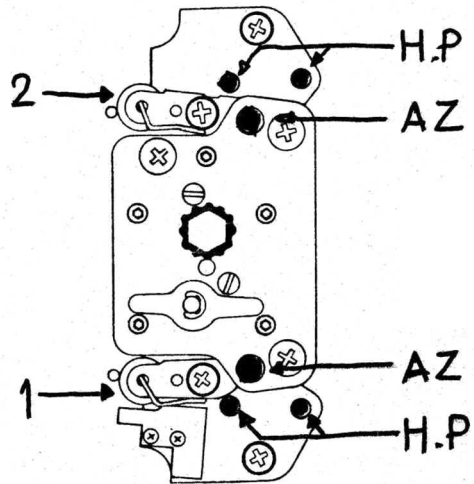
Fig. 5.4 Adjustments for the pinch rollers
