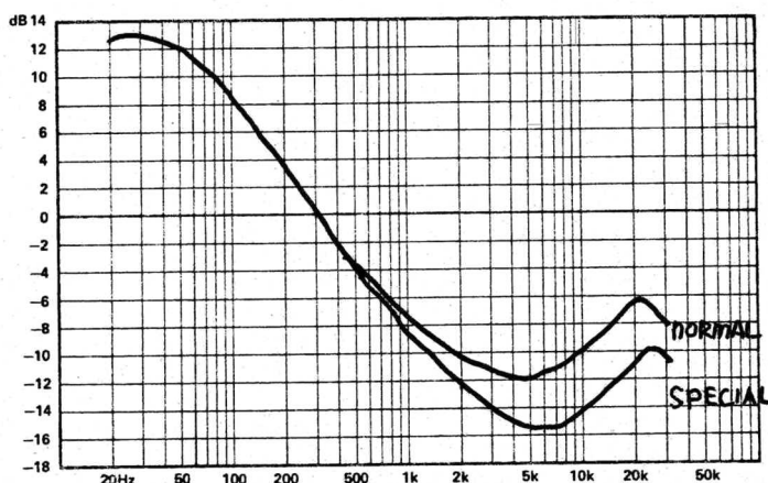
Fig. 4.5 Playback correction
