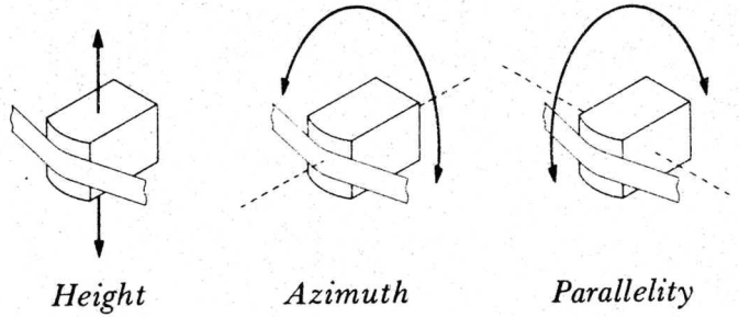
Fig. 5.1 Head adjustments
