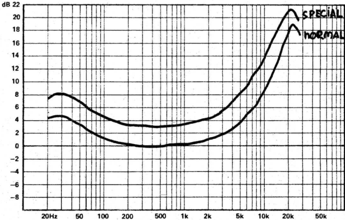
Fig. 4.7 Record correction
