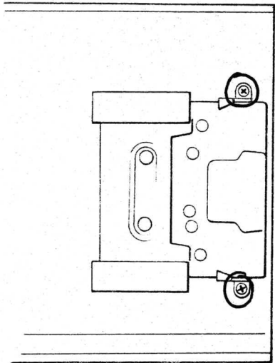
Fig. 3.8 Screws for head bridge guide brackets
