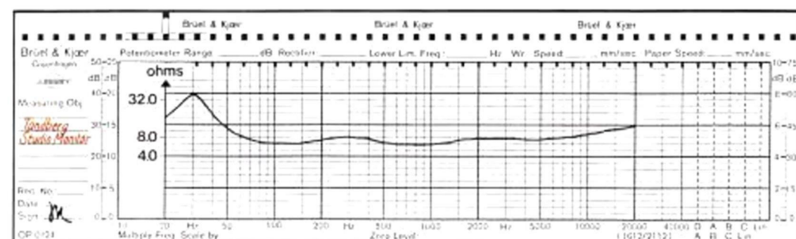
Impedance characteristic (ohms).
