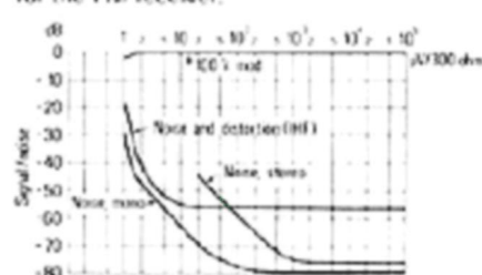
Signal/noise ratio in stereo and mono for the FM receiver.
