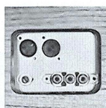
3. DIN-contacts for radio recording and playback through radio or for external loudspeakers. An output for Free Head (4 track) or Monitor (2 track).
