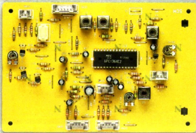
Secam-Decoder
