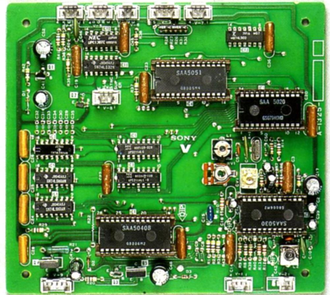
Videotext-Decoder
