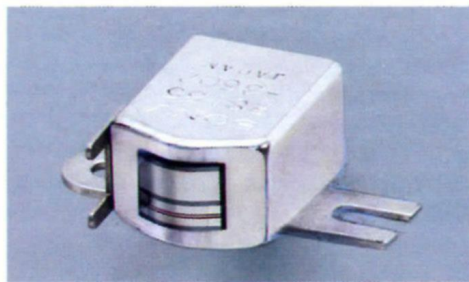
Sony's Sendust and Ferrite record/play head.
