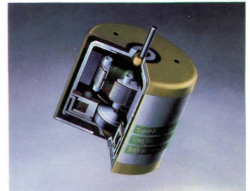
Sony's stable, durable Tri-Duty DC Servo Motor.
