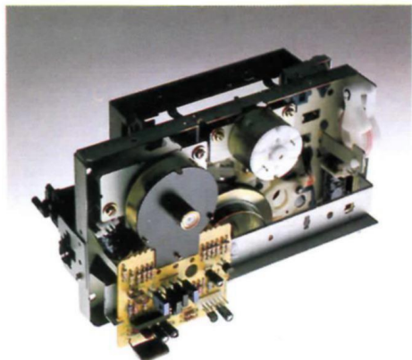
Sony's two-motor tape drive system.
