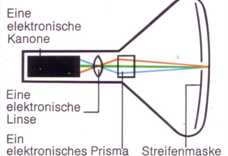
TRINITRON-Röhre
