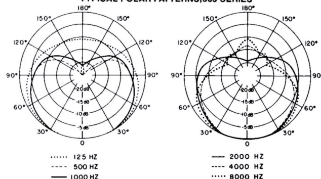
TYPICAL POLAR PATTERNS, 565 SERIES
