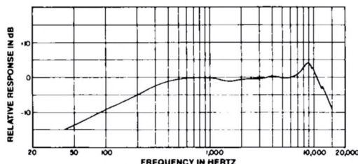
TYPICAL FREQUENCY RESPONSE, SM11
