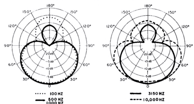
TYPICAL POLAR PATTERNS, SM87
