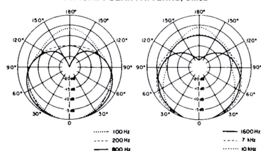
TYPICAL POLAR PATTERNS, SM62
