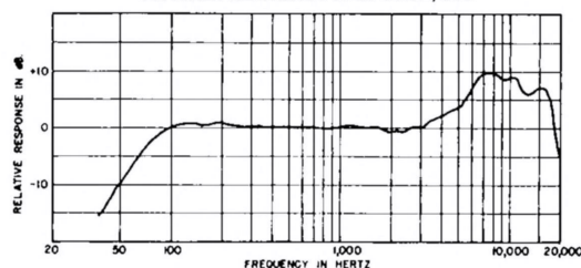
TYPICAL FREQUENCY RESPONSE, 838
