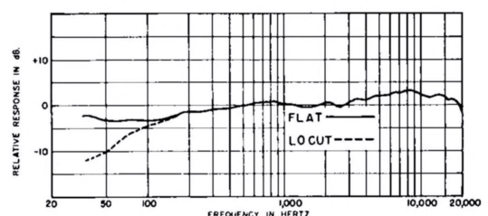
TYPICAL FREQUENCY RESPONSE, SM91
