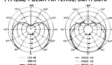
TYPICAL POLAR PATTERNS, SM77, SM78
