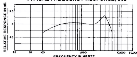
TYPICAL FREQUENCY RESPONSE, 562
