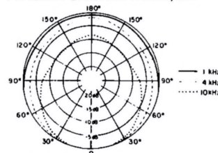
TYPICAL POLAR PATTERNS, 578
