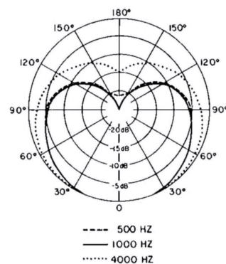
TYPICAL POLAR PATTERN, 512
