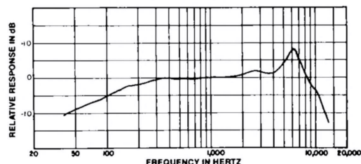
TYPICAL FREQUENCY RESPONSE, SM51
