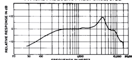
TYPICAL FREQUENCY RESPONSE, 572G
