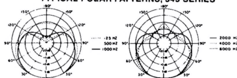
TYPICAL POLAR PATTERNS, 545 SERIES
