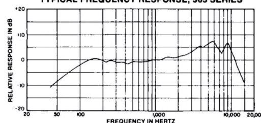
TYPICAL FREQUENCY RESPONSE, 565 SERIES
