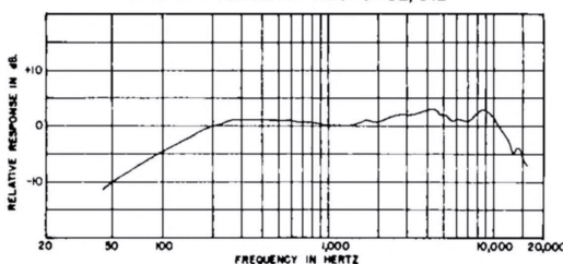
TYPICAL FREQUENCY RESPONSE, 512
