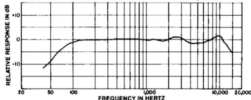
TYPICAL FREQUENCY RESPONSE, 578
