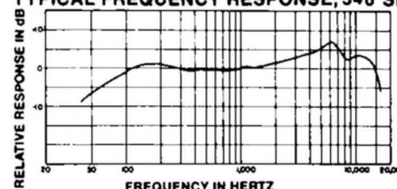
TYPICAL FREQUENCY RESPONSE, 546 SERIES
