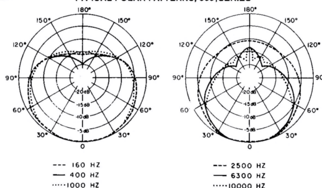
TYPICAL POLAR PATTERNS, 588 SERIES
