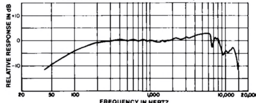
TYPICAL FREQUENCY RESPONSE, 579SB
