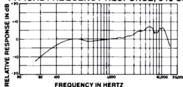
TYPICAL FREQUENCY RESPONSE, 545 SERIES
