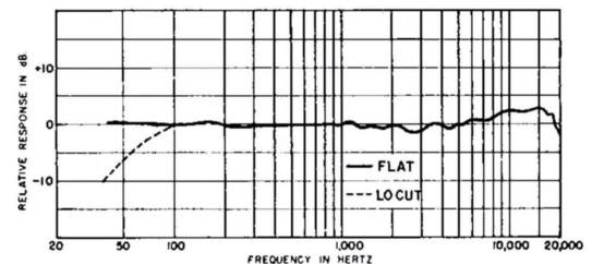
TYPICAL FREQUENCY RESPONSE, SM90
