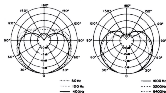
TYPICAL POLAR PATTERNS, SM5B
