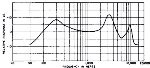
TYPICAL HEADPHONE RESPONSE, 512
