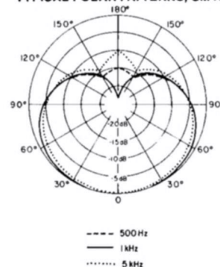
TYPICAL POLAR PATTERNS, SM18
