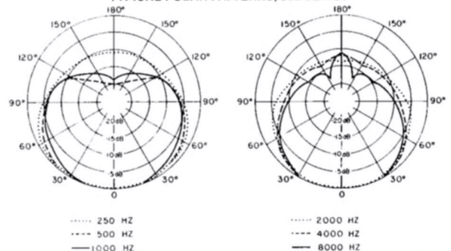
TYPICAL POLAR PATTERNS, 585 SERIES
