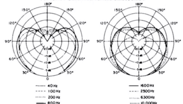
TYPICAL POLAR PATTERNS SM53, SM54
