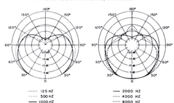
TYPICAL POLAR PATTERNS, SM56, SM57
