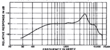
TYPICAL FREQUENCY RESPONSE, 561
