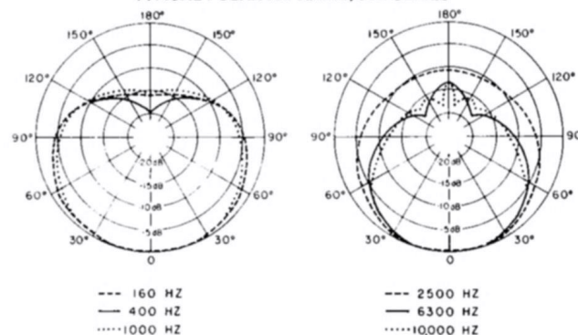
TYPICAL POLAR PATTERNS, 588 SERIES
