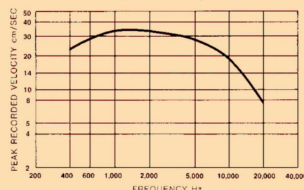
TRACKABILITY CHART (at 1 Gram)
