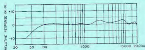
FREQ. RESPONSE
