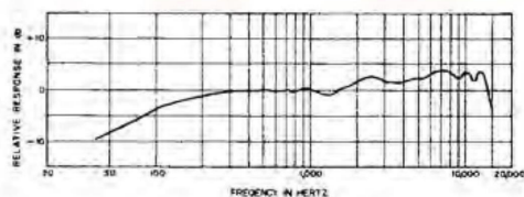
FREQ. RESPONSE
