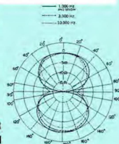
POLAR PATTERN
