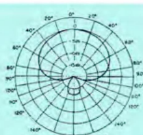
POLAR PATTERN
