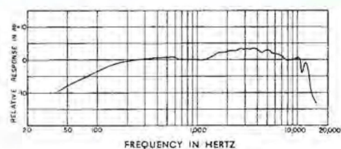
FREQ. RESPONSE
