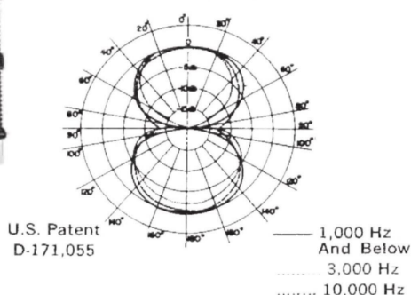
DIRECTIONAL PATTERN
