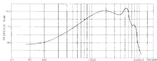
FREQUENCY IN HERTZ FREQUENCY RESPONSE
