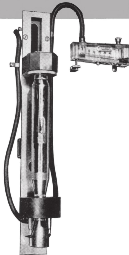
Enlarged View of Hydrogen-Filled Coupler
