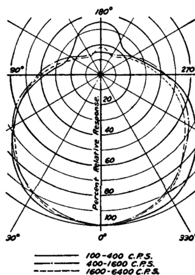
Horizontal Polar Response Series 556 Microphones
