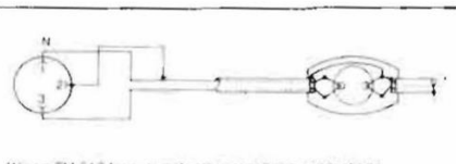
Wiring TM 513 for symmetrical microphone connections
