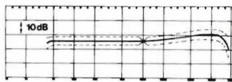
Rated frequency response (with tolerance field)
