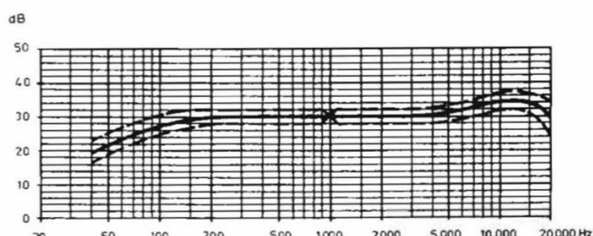
Rated frequency response (with tolerance field) MKH 816 P 48, measuring distance 1 m. Each microphone is accompanied by the original test certificate measured from 50 to 20,000 Hz
