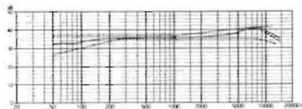
ME 80 Frequency Response Curve
