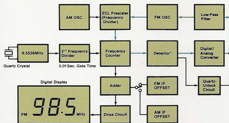
BLOCK DIAGRAM OF SANSUI DIGITALLY QUARTZ-LOCKED TUNING
