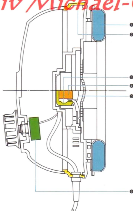
① EAR CUSHION ② HOUSING ③ YOK ④ PERMANENT MAGNET ⑤ POLYESTER DIAPHRAGM ASSEMBLY ⑥ VOLUME CONTROL
