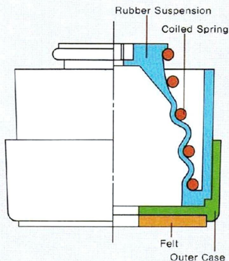
Cross Section Diagram of the Cabinet Suspension
