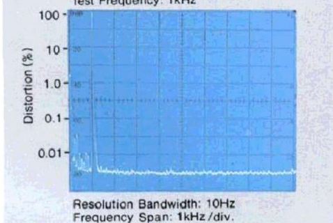
HARMONIC DISTORTION (Distortion Spectrum) 250mW G-9000 Input Terminal: Aux Output Level: 250mW Test Frequency: 1kHz
