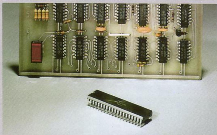
The Large-Scale Integrated Circuit (LSI) you see in the foreground now compactly houses all the discrete parts, wiring and ICs grouped behind it. This Sansui innovation assures computer-grade reliability in our Digitally Quartz-Locked Tuning System.
