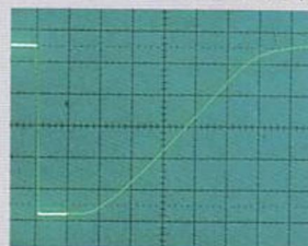
SLEW RATE & RISE TIME (Power Amp)
