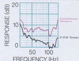
LOW-FREQUENCY RESONANCE RESPONSE
