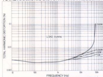
TOTAL HARMONIC DISTORTION vs FREQUENCY
