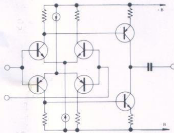
Linear complete-mirrored parallel push-pull circuitry
