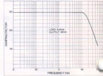
DAMPING FACTOR vs FREQUENCY
