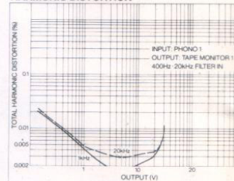
PHONO (MM) OUTPUT vs TOTAL HARMONIC DISTORTION
