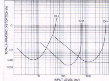
PHONO INPUT LEVEL vs OUTPUT DISTORTION
