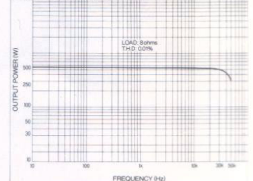
POWER BAND WIDTH
