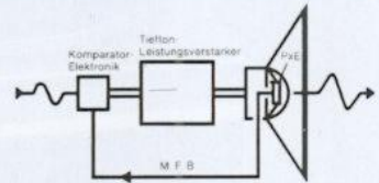
Motional-Feed-Back-System
