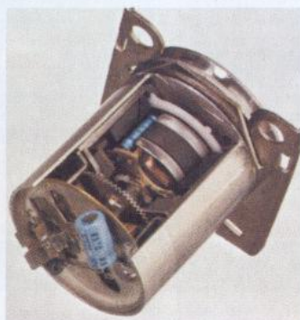
Direct-Drive-Motor
